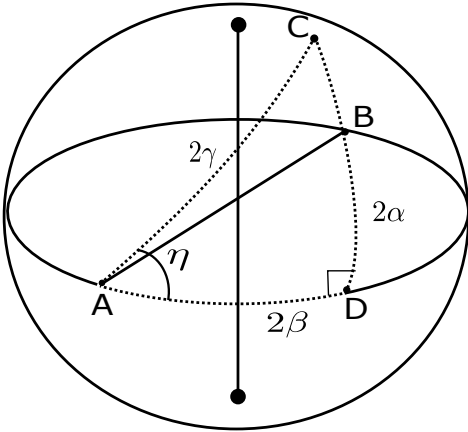
Fig. 2. Poincaré sphere
