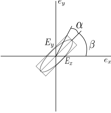
Fig. 1. Polarization ellipse
