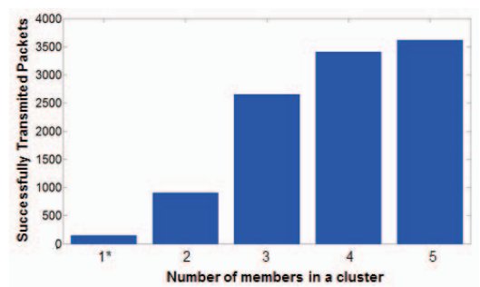
Figure 11. Successfully transmissions at 15s transmission time.
