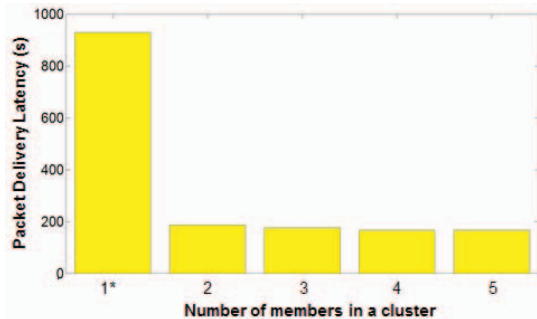
Figure 15. Delay at 7s transmission time.
