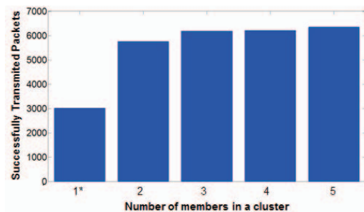
Figure 8. Successfully transmissions at 7s transmission time.
