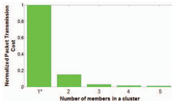
Figure 13. Normalized transmission cost at 15s transmission time.
