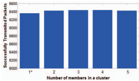
Figure 5. Successfully transmissions at 1s transmission time.
