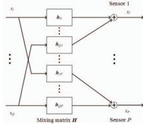
Figure 2. General case – MIMO system Q transmitters and P receivers
