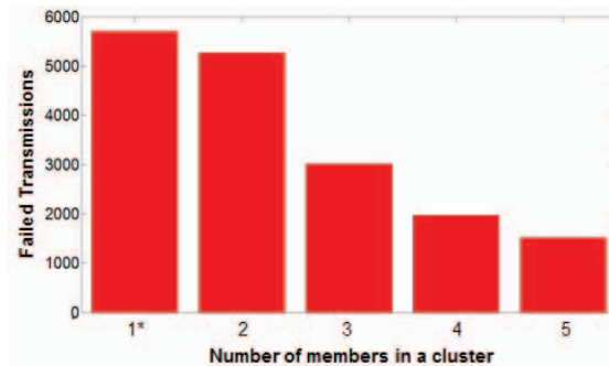
Figure 12. Failed transmissions at 15s transmission time.
