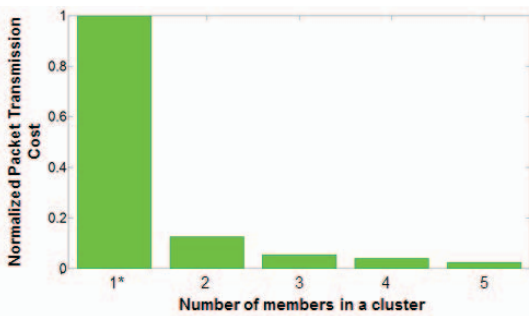
Figure 10. Normalized transmission cost at 7s transmission time.
